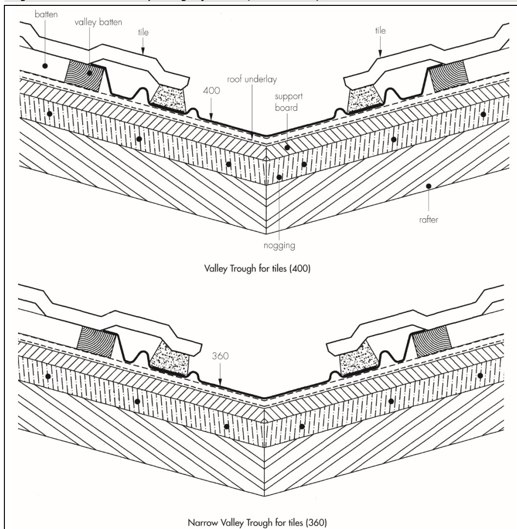
Figure 1 Klober GRP Valley Troughs for Tiles (400 and 360) – Batten Fix
